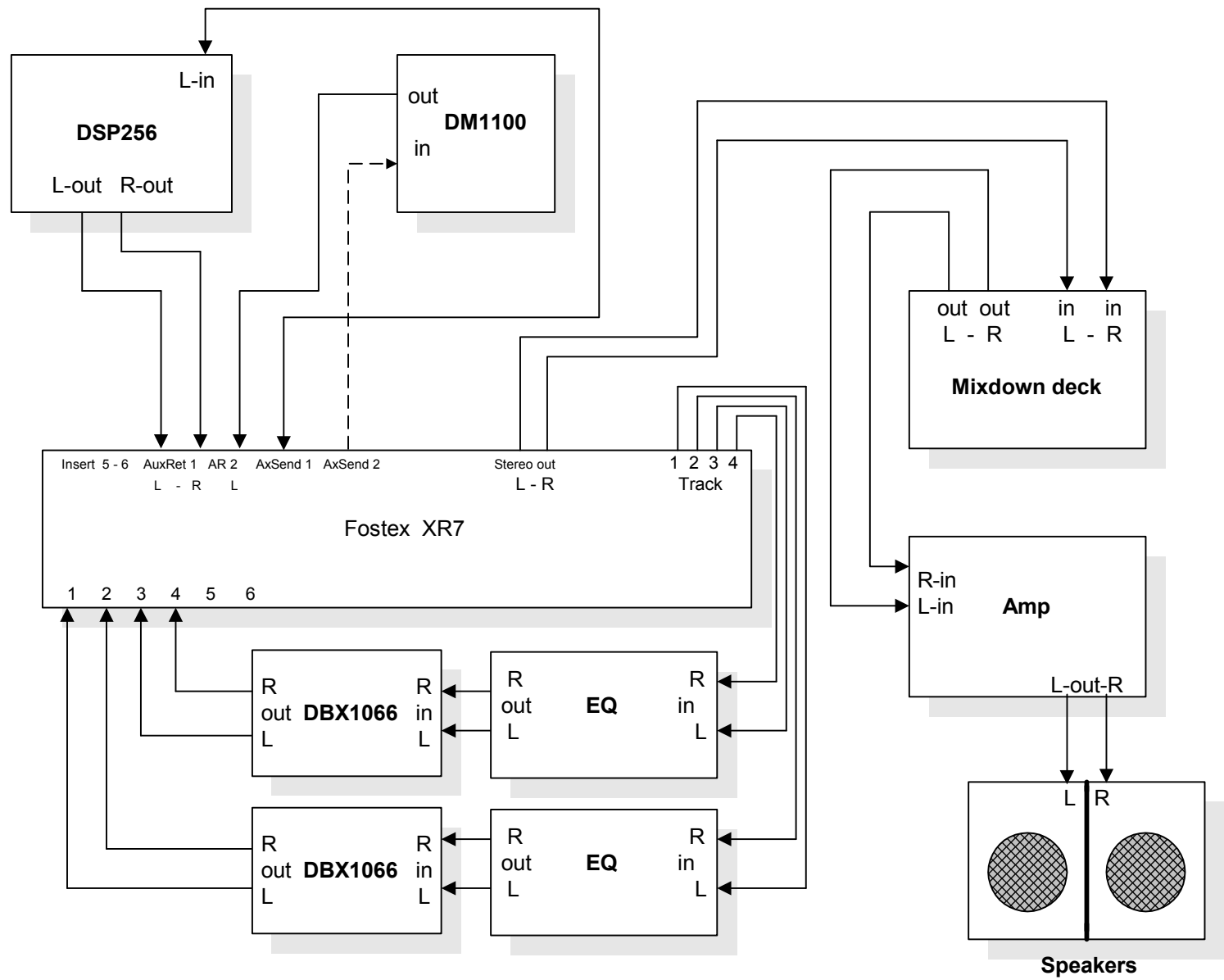
Diagram #3d : This setup could also be run through the effects loops, but either way a patch bay would probably be the easiest way to manage the changeover from recording to mixdown.
